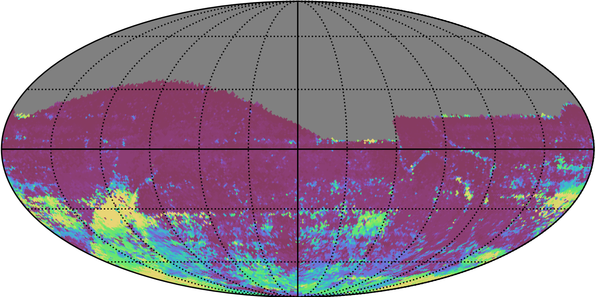
ddf_acor_sf30_lsf40_lsr20_v3.4_10yrs All sky r band: 75th Percentile Intranight Timespan
