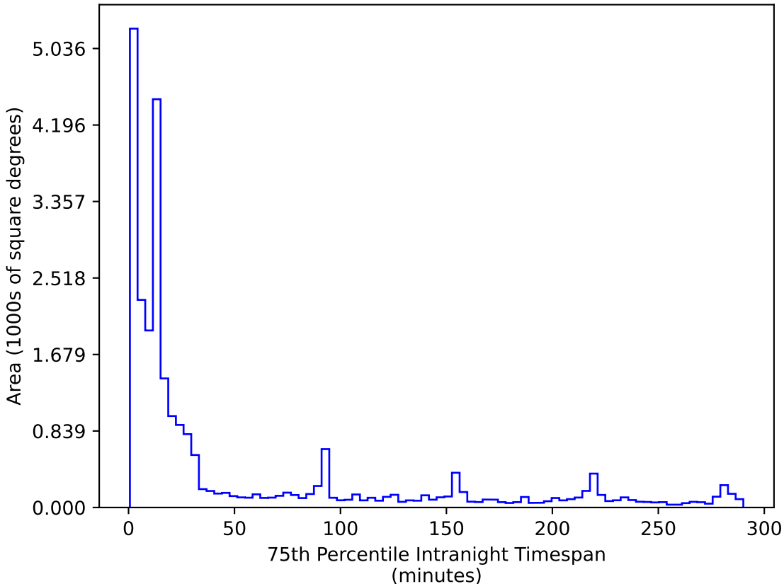
ddf_acor_sf30_lsf40_lsr20_v3.4_10yrs All sky r band: 75th Percentile Intranight Timespan
