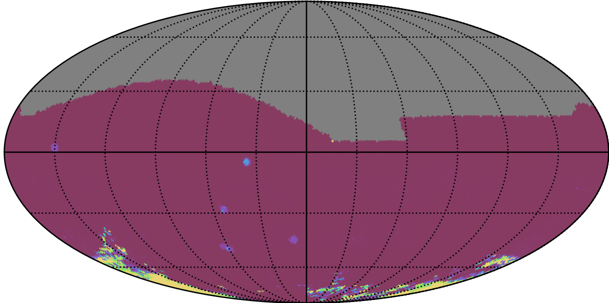
ddf_acor_sf30_lsf40_lsr20_v3.4_10yrs All sky iz bands: 75th Percentile Intranight Timespan
