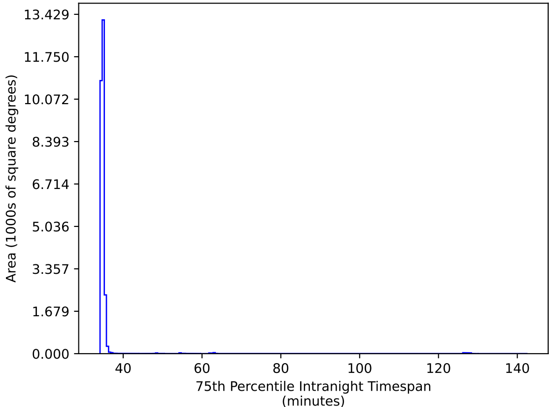
ddf_acor_sf30_lsf40_lsr20_v3.4_10yrs All sky iz bands: 75th Percentile Intranight Timespan
