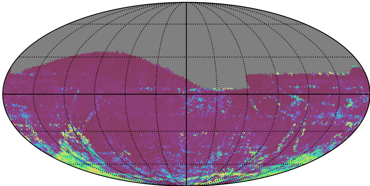
ddf_acor_sf30_lsf40_lsr20_v3.4_10yrs All sky i band: 75th Percentile Intranight Timespan
