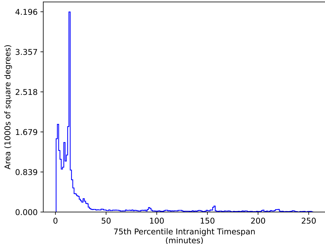
ddf_acor_sf30_lsf40_lsr20_v3.4_10yrs All sky i band: 75th Percentile Intranight Timespan
