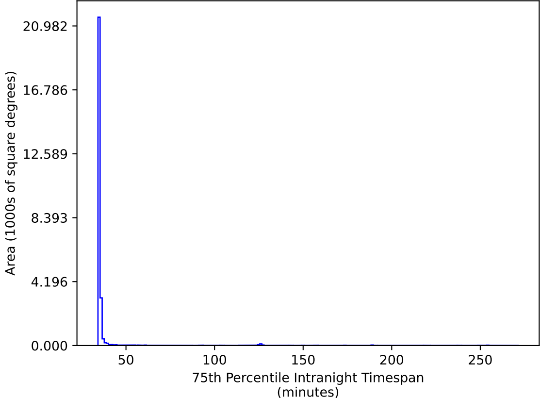
ddf_acor_sf30_lsf40_lsr20_v3.4_10yrs All sky gr bands: 75th Percentile Intranight Timespan
