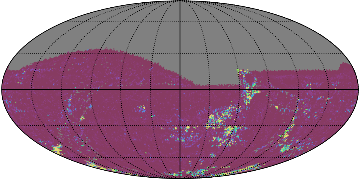
ddf_acor_sf30_lsf40_lsr20_v3.4_10yrs All sky g band: 75th Percentile Intranight Timespan
