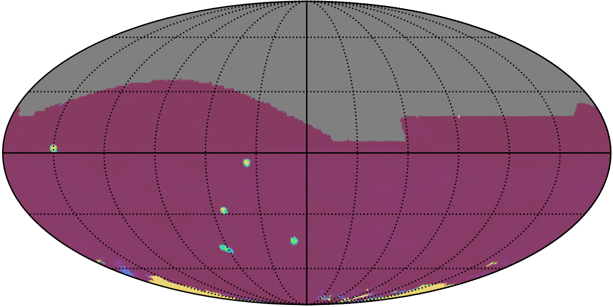
ddf_acor_sf30_lsf40_lsr20_v3.4_10yrs All sky all bands: 75th Percentile Intranight Timespan
