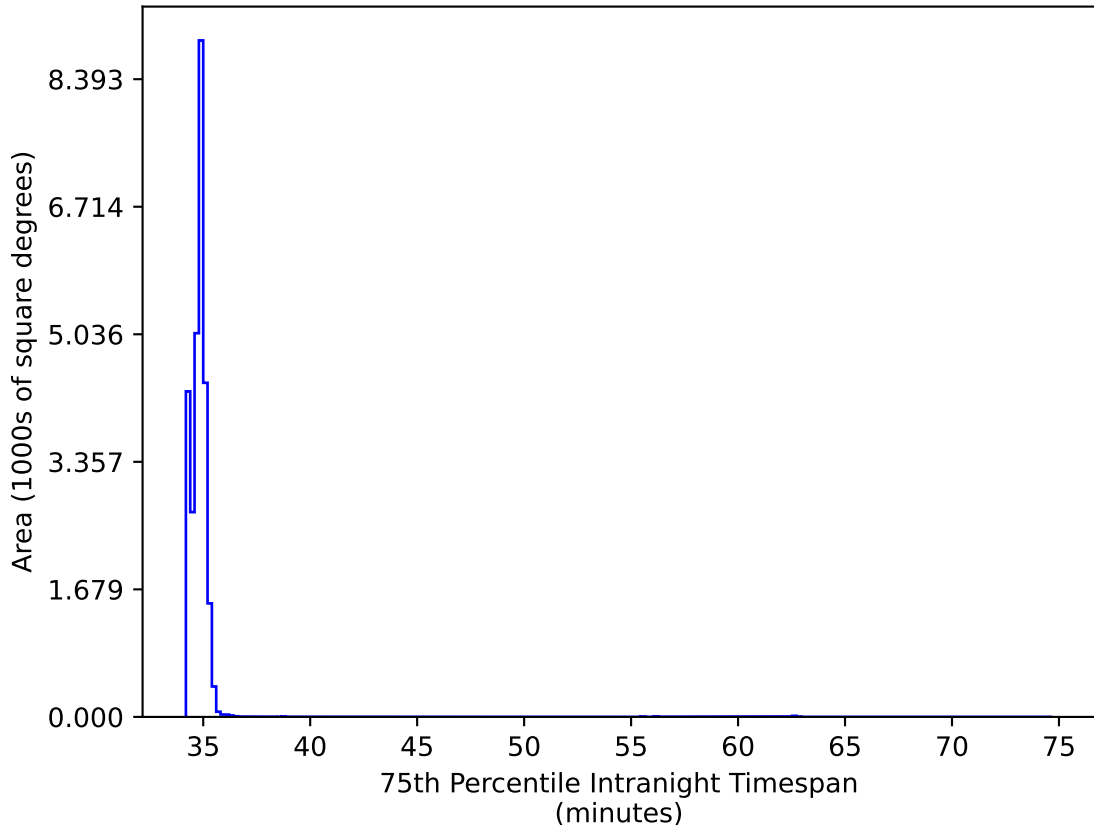
ddf_acor_sf30_lsf40_lsr20_v3.4_10yrs All sky all bands: 75th Percentile Intranight Timespan
