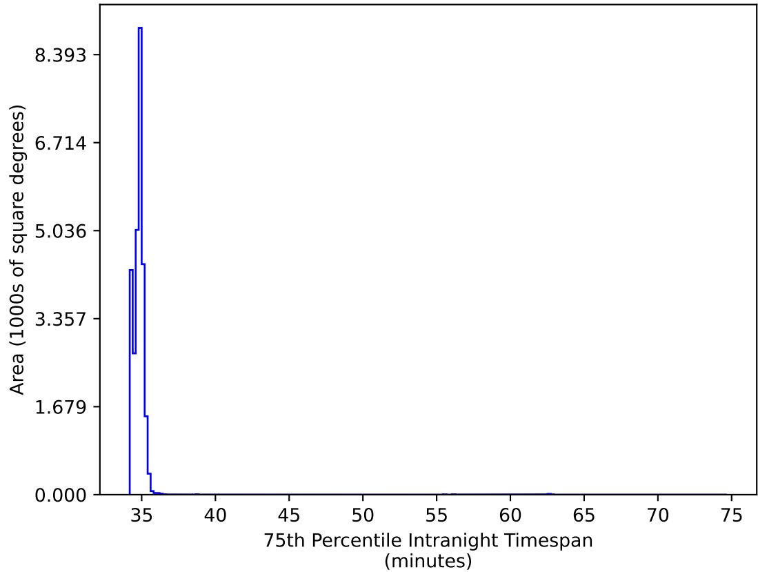
ddf_acor_sf30_lsf40_lsr20_v3.4_10yrs All sky: 75th Percentile Intranight Timespan
