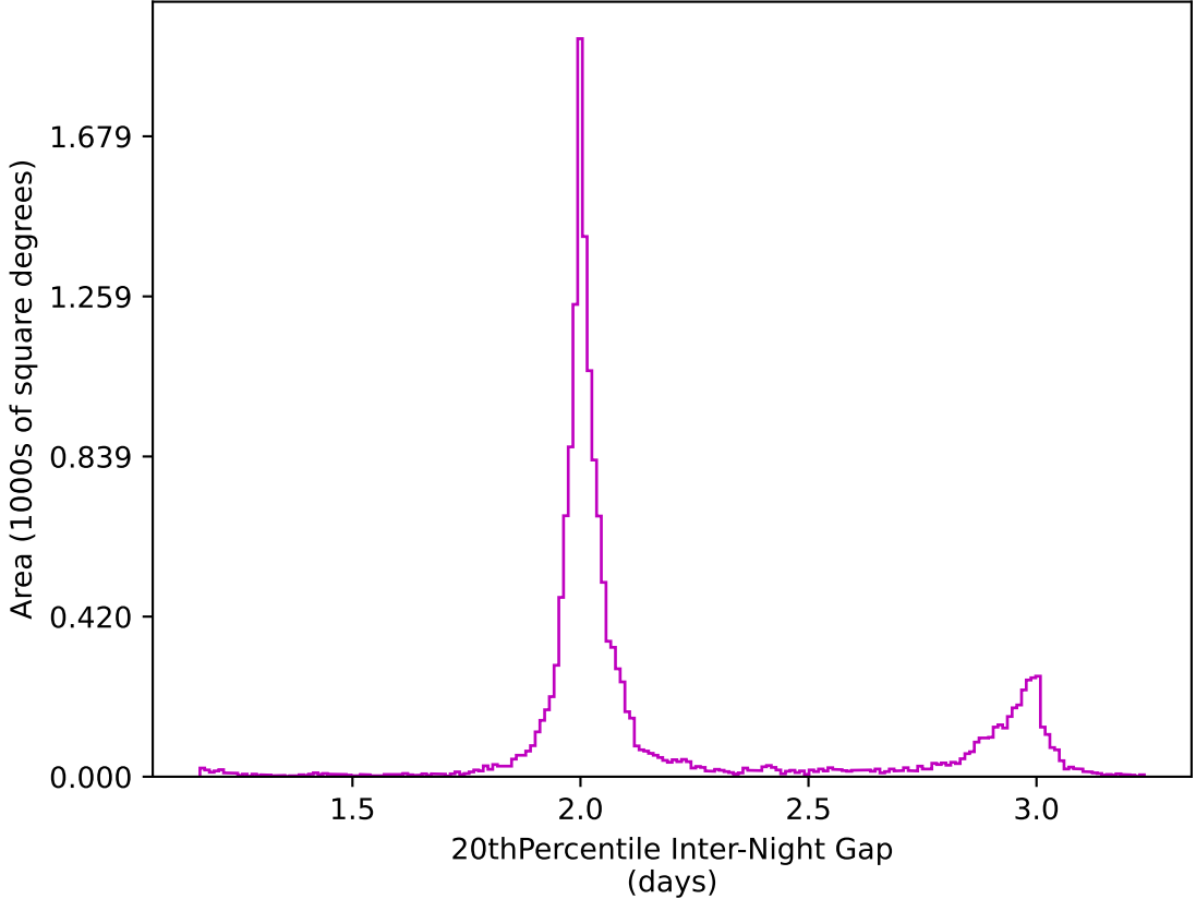
ddf_acor_sf30_lsf40_lsr20_v3.4_10yrs WFD z band: 20thPercentile Inter-Night Gap
