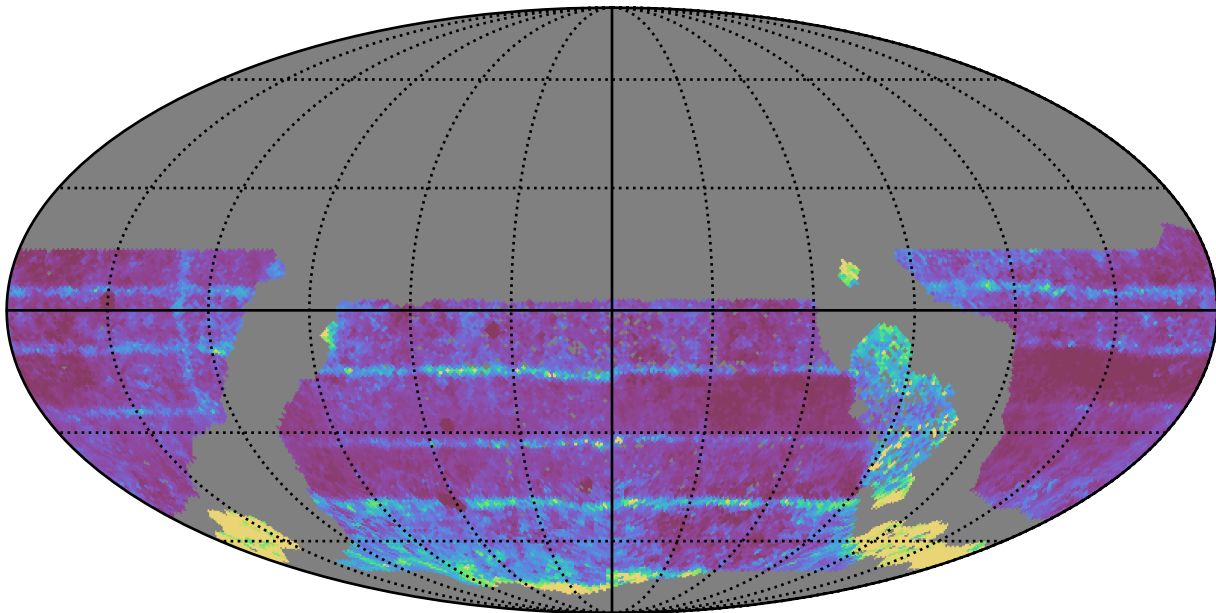
ddf_acor_sf30_lsf40_lsr20_v3.4_10yrs WFD all bands: 20thPercentile Inter-Night Gap
