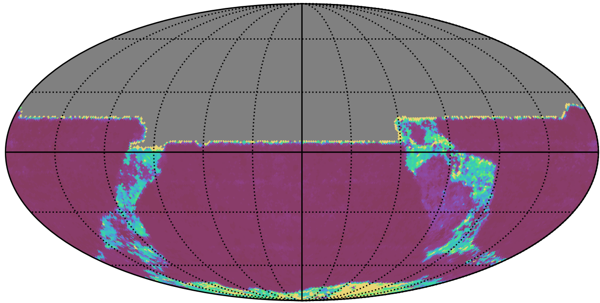
ddf_acor_sf30_lsf40_lsr20_v3.4_10yrs All sky y band: 20thPercentile Inter-Night Gap
