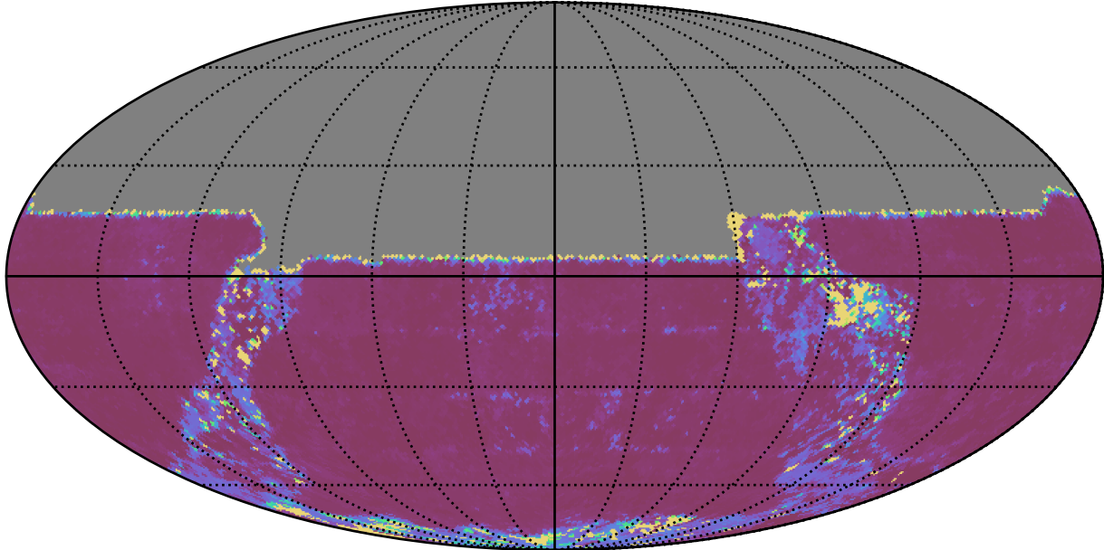
ddf_acor_sf30_lsf40_lsr20_v3.4_10yrs All sky u band: 20thPercentile Inter-Night Gap
