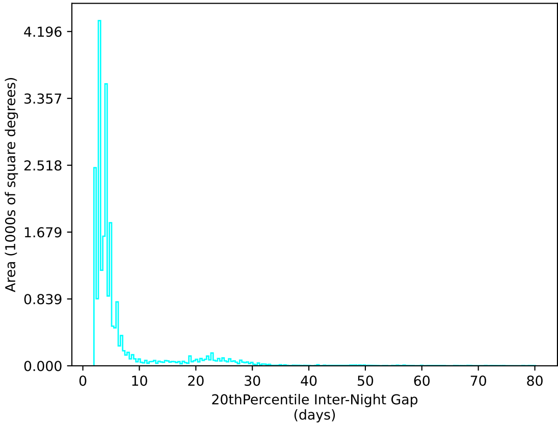
ddf_acor_sf30_lsf40_lsr20_v3.4_10yrs All sky u band: 20thPercentile Inter-Night Gap
