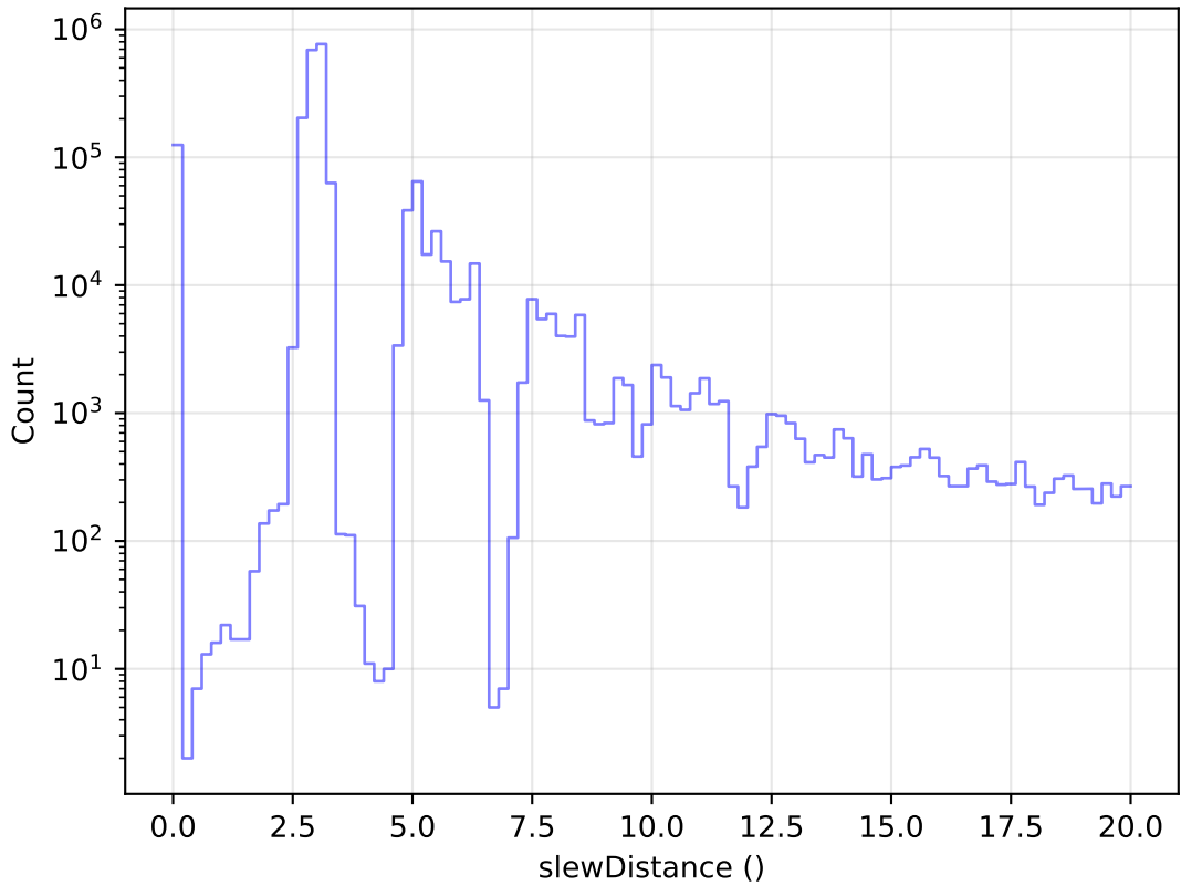
ddf_acor_sf30_lsf40_lsr20_v3.4_10yrs All visits: Zoom Slew Distance Histogram
