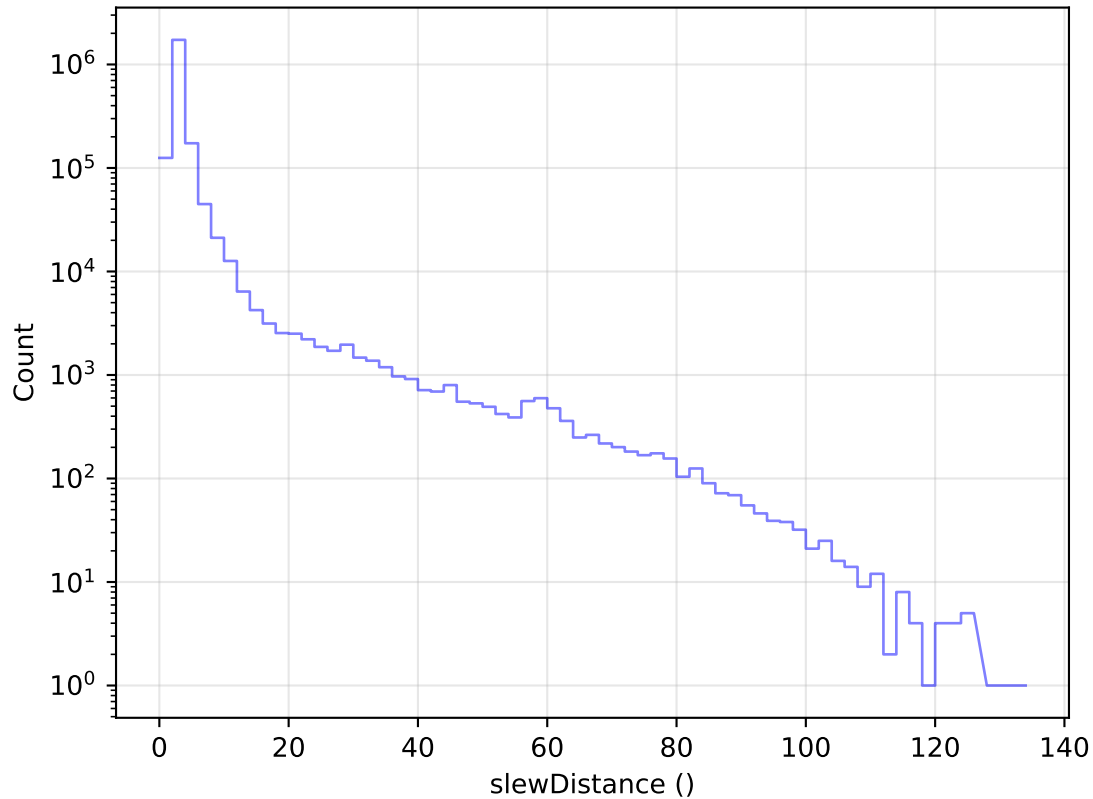
ddf_acor_sf30_lsf40_lsr20_v3.4_10yrs All visits: Slew Distance Histogram
