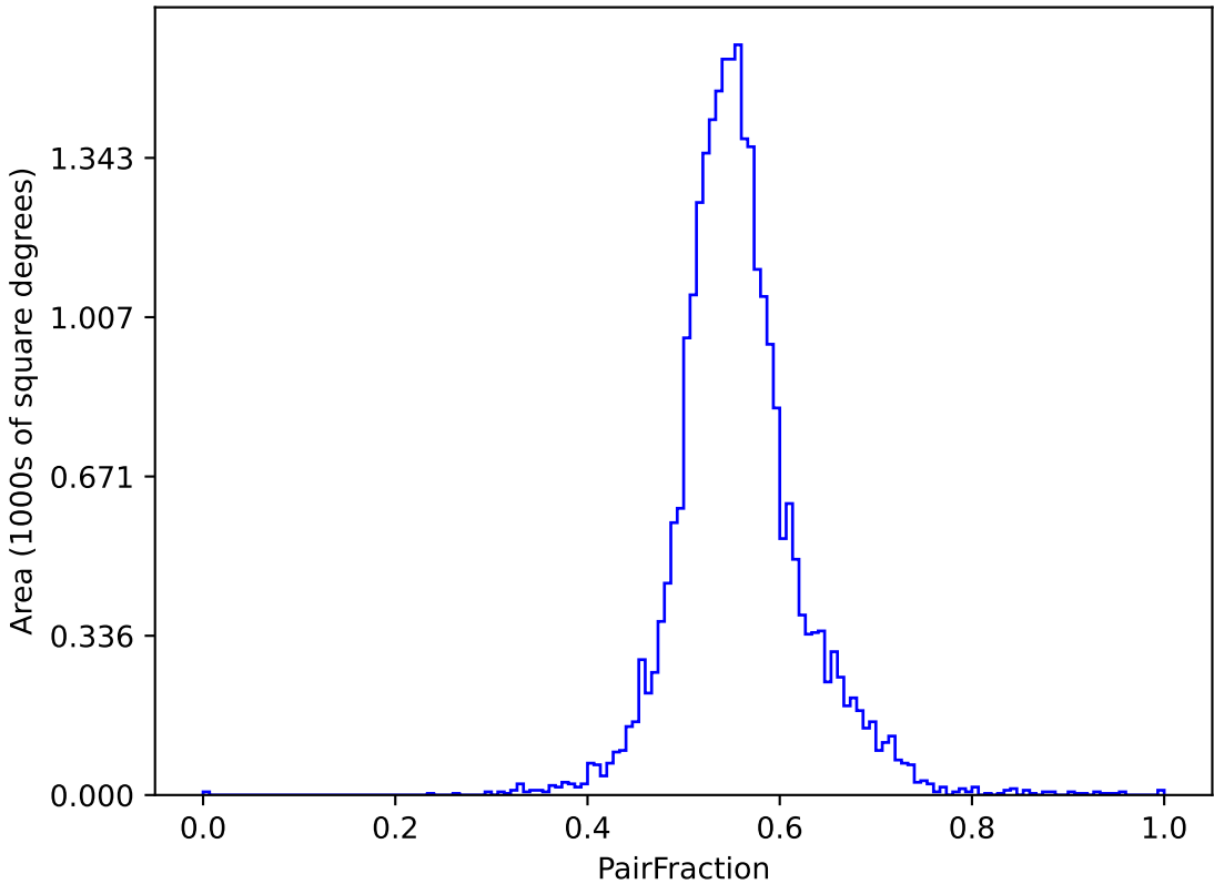
ddf_acor_sf30_lsf40_lsr20_v3.4_10yrs (g or r or i): PairFraction
