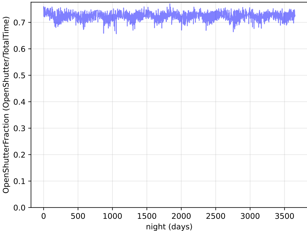
ddf_acor_sf30_lsf40_lsr20_v3.4_10yrs : OpenShutterFraction
