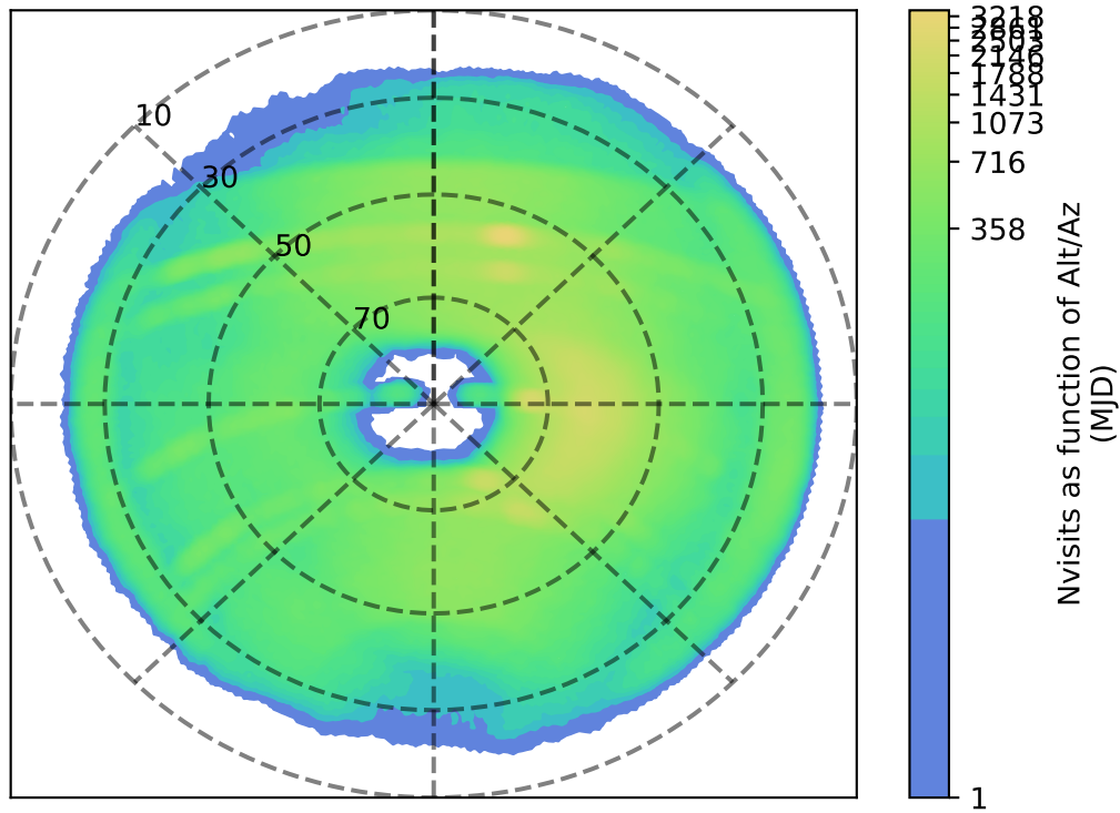
ddf_acor_sf30_lsf40_lsr20_v3.4_10yrs z: Nvisits as function of Alt/Az
