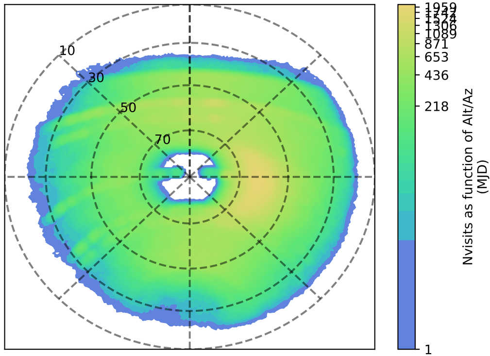
ddf_acor_sf30_lsf40_lsr20_v3.4_10yrs y: Nvisits as function of Alt/Az
