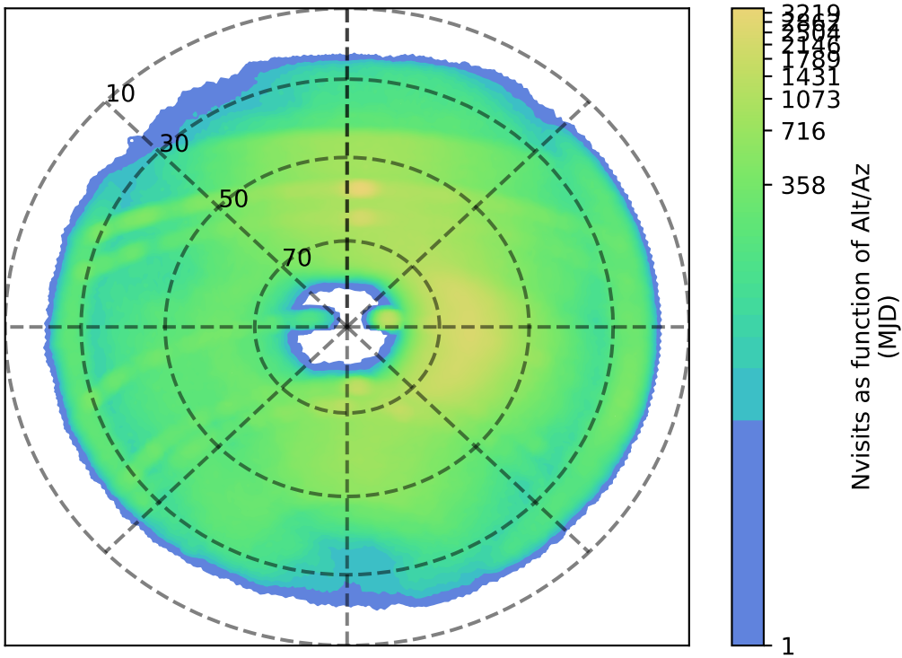
ddf_acor_sf30_lsf40_lsr20_v3.4_10yrs i: Nvisits as function of Alt/Az
