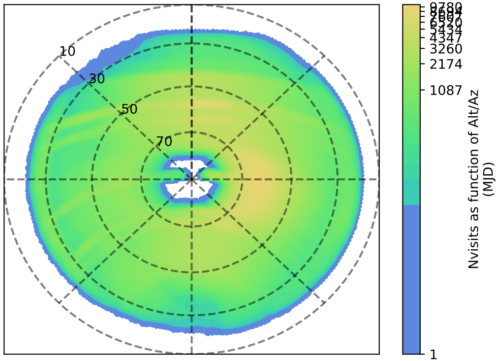
ddf_acor_sf30_lsf40_lsr20_v3.4_10yrs : Nvisits as function of Alt/Az
