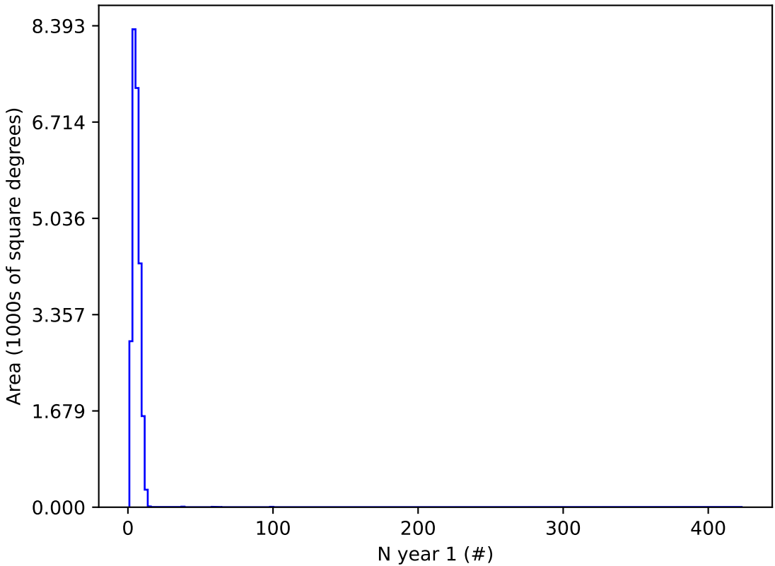
ddf_acor_sf30_lsf40_lsr20_v3.4_10yrs u and night < 365: N year 1
