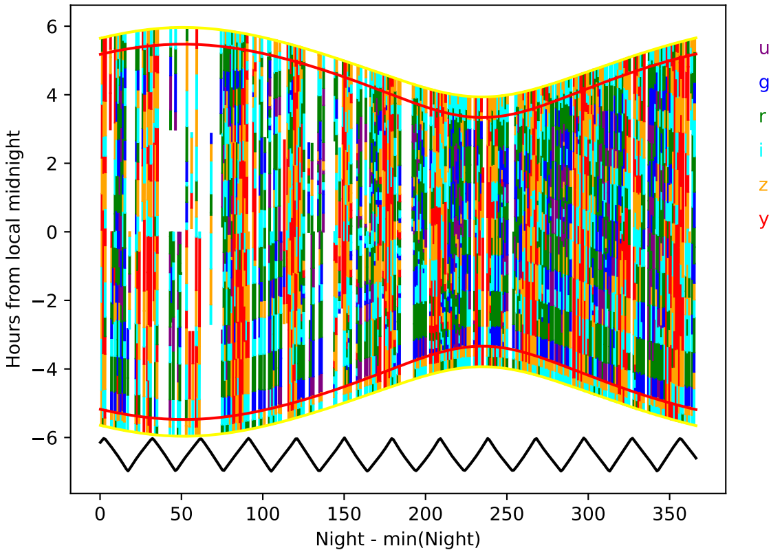
ddf_acor_sf30_lsf40_lsr20_v3.4_10yrs year 9-10: Hourglass
