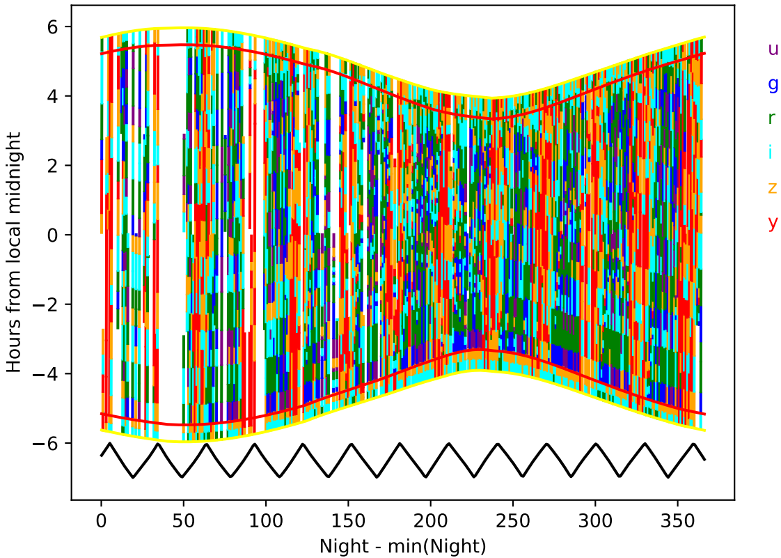
ddf_acor_sf30_lsf40_lsr20_v3.4_10yrs year 6-7: Hourglass
