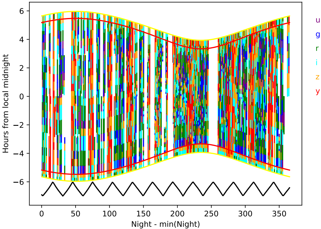
ddf_acor_sf30_lsf40_lsr20_v3.4_10yrs year 5-6: Hourglass
