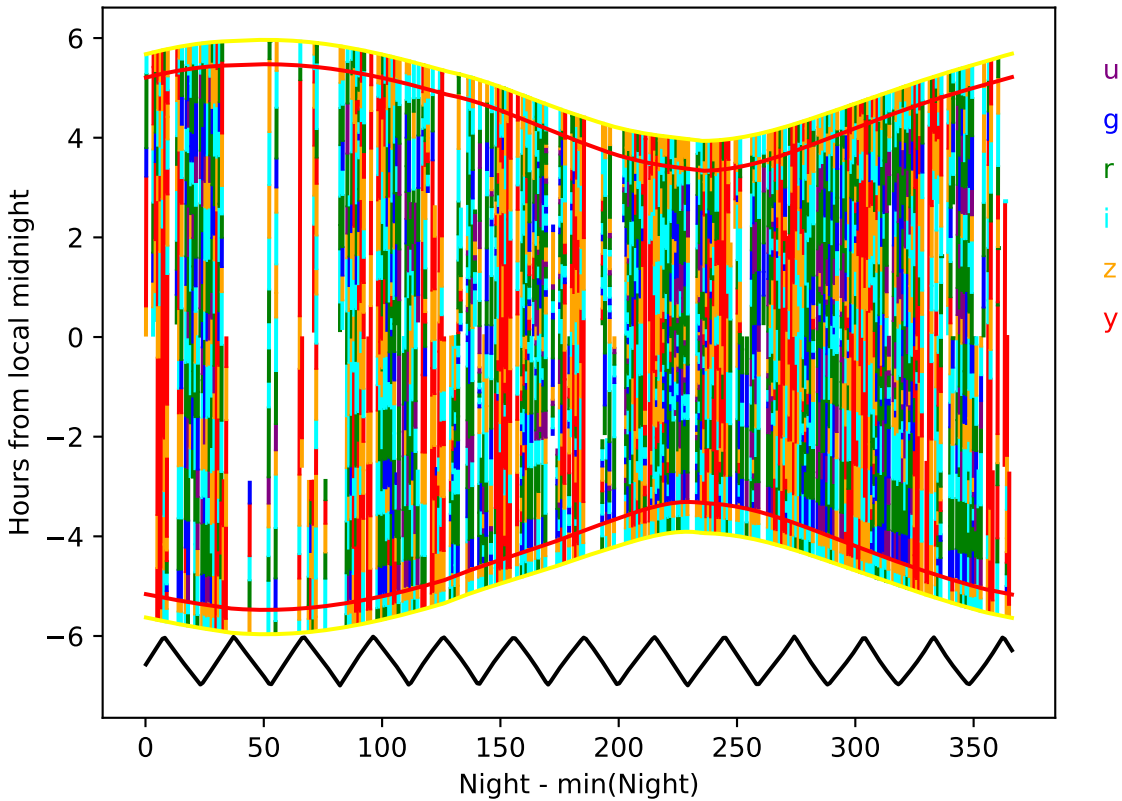
ddf_acor_sf30_lsf40_lsr20_v3.4_10yrs year 3-4: Hourglass
