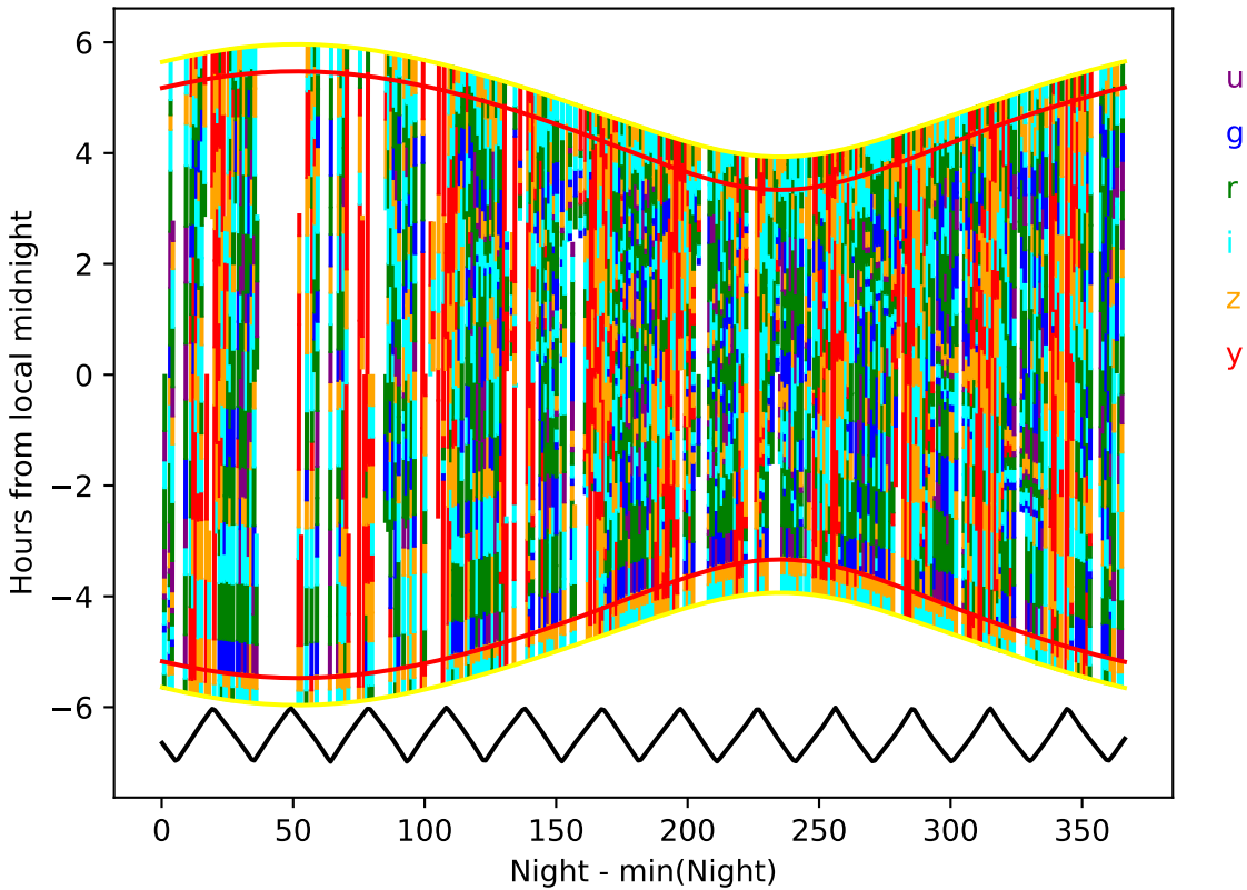
ddf_acor_sf30_lsf40_lsr20_v3.4_10yrs year 2-3: Hourglass
