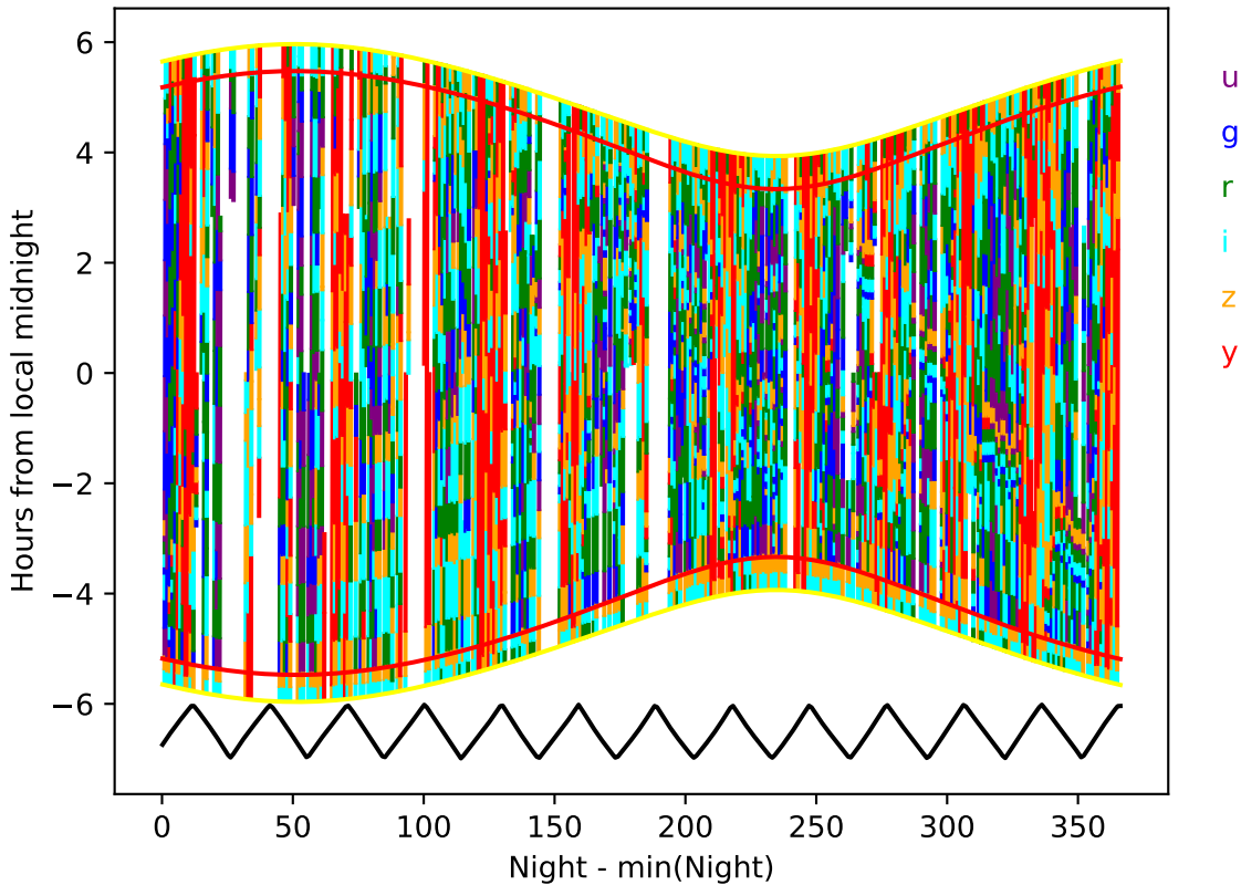
ddf_acor_sf30_lsf40_lsr20_v3.4_10yrs year 0-1: Hourglass
