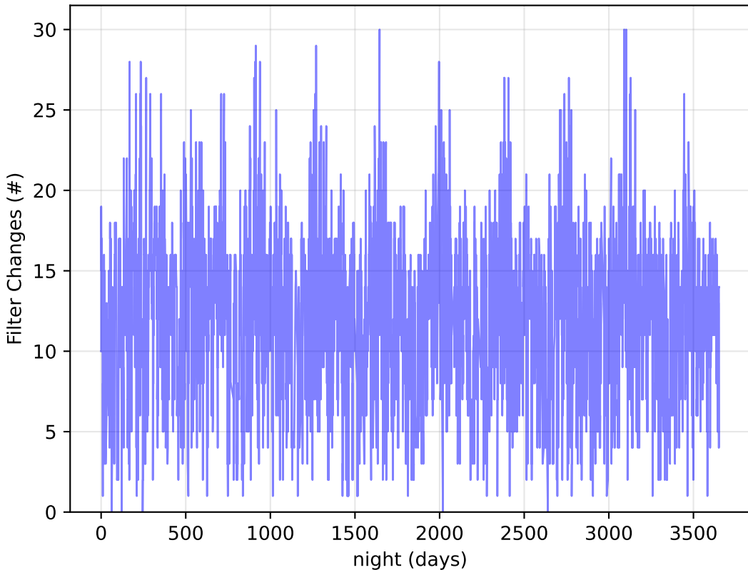
ddf_acor_sf30_lsf40_lsr20_v3.4_10yrs : Filter Changes
