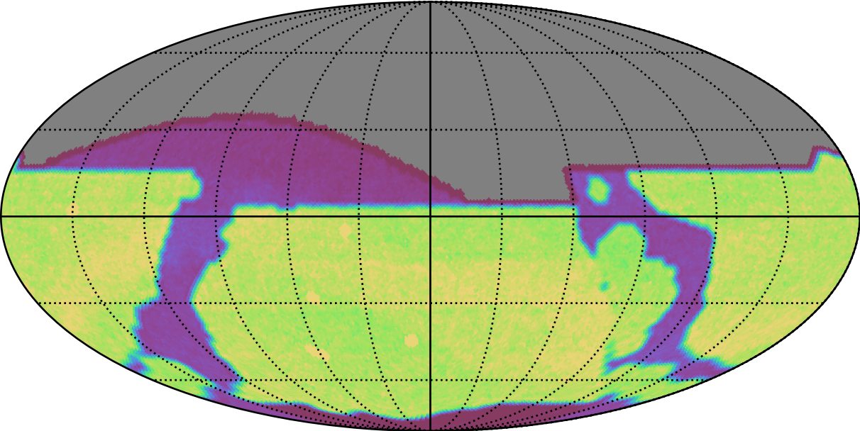
ddf_acor_sf30_lsf40_lsr20_v3.4_10yrs : Count observationStartMJD
