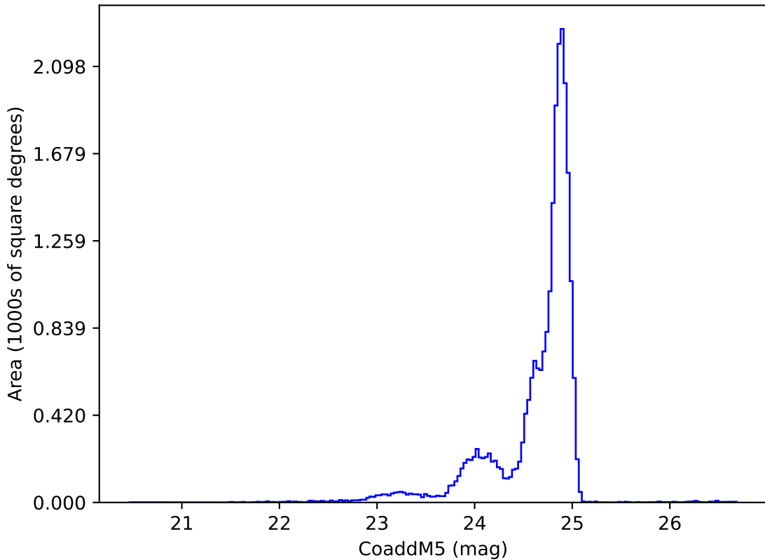
ddf_acor_sf30_lsf40_lsr20_v3.4_10yrs y: CoaddM5
