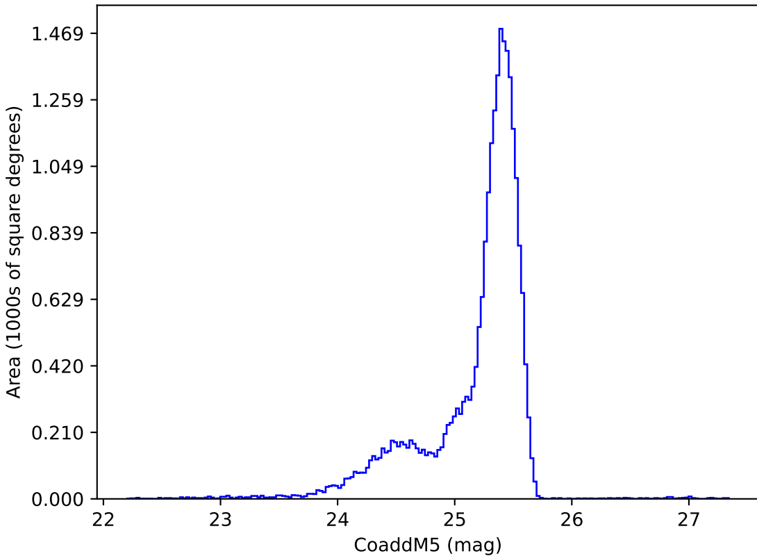
ddf_acor_sf30_lsf40_lsr20_v3.4_10yrs u: CoaddM5
