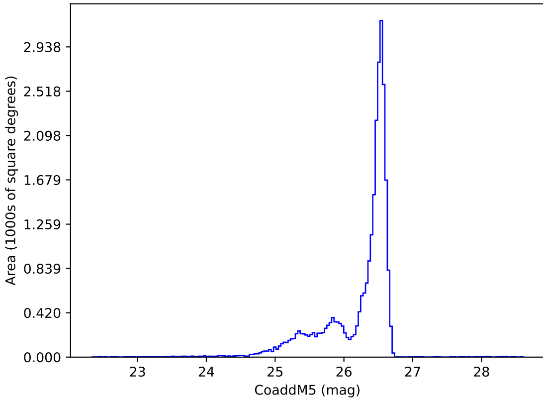
ddf_acor_sf30_lsf40_lsr20_v3.4_10yrs i: CoaddM5
