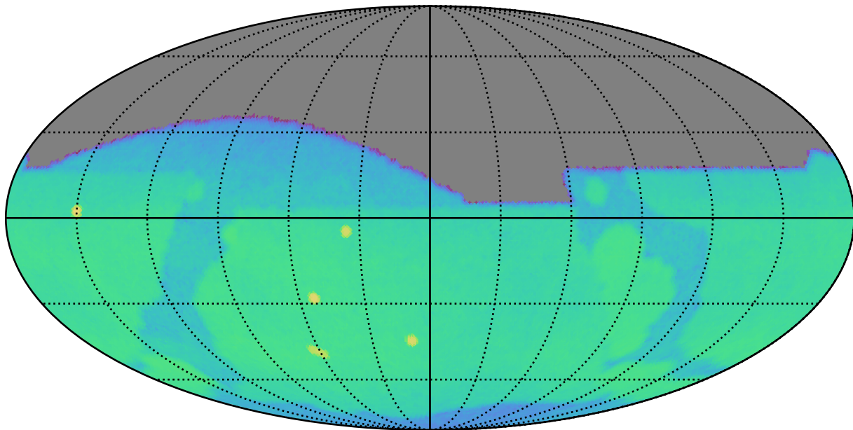
ddf_acor_sf30_lsf40_lsr20_v3.4_10yrs g: CoaddM5
