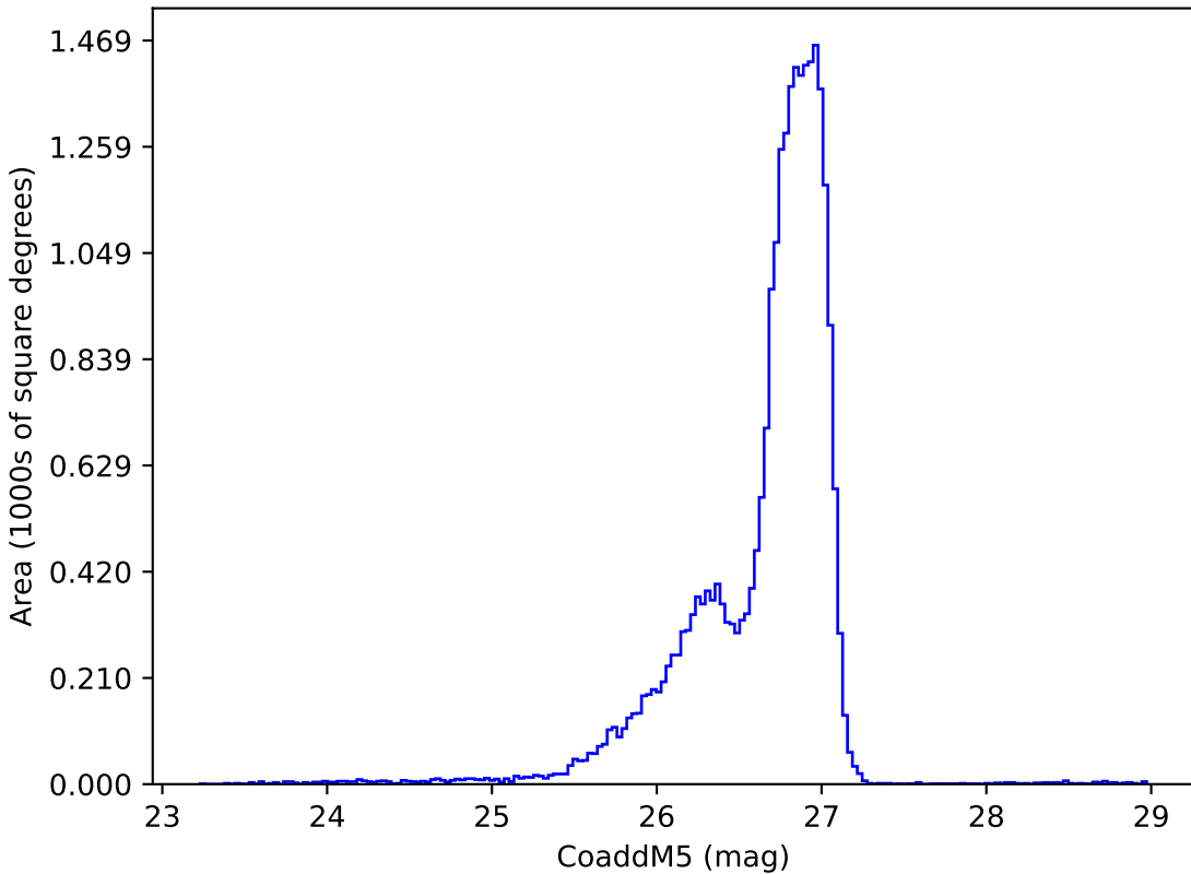
ddf_acor_sf30_lsf40_lsr20_v3.4_10yrs g: CoaddM5
