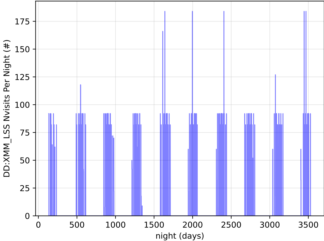
ddf_acor_sf30_lsf40_lsr20_v3.4_10yrs all bands: DD:XMM_LSS Nvisits Per Night
