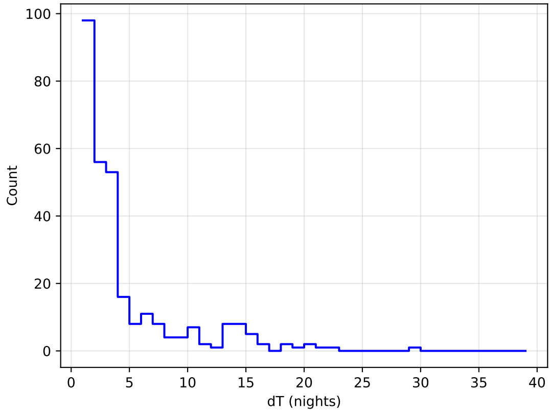
ddf_acor_sf30_Isf40_Isr20_v3.4_10yrs all bands: DD:XMM_LSS Delta Nights Histogram
