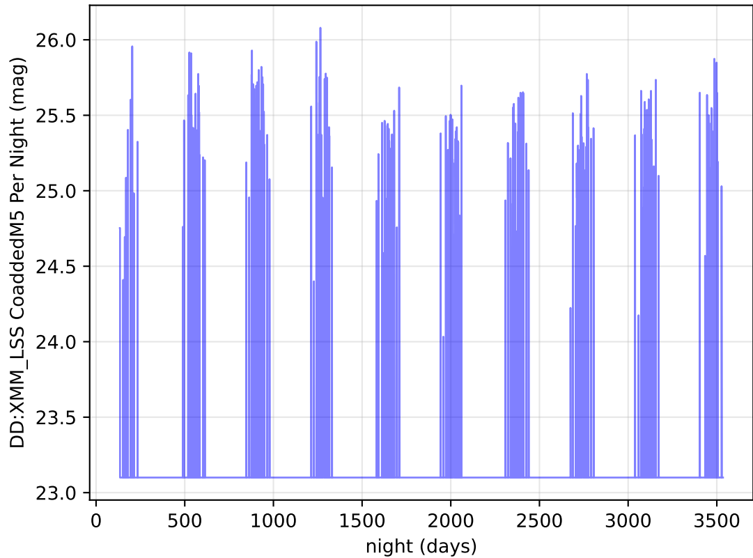
ddf_acor_sf30_lsf40_lsr20_v3.4_10yrs i band: DD:XMM_LSS CoaddedM5 Per Night
