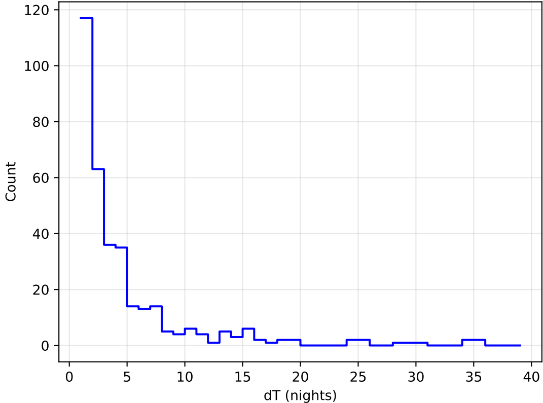
ddf_acor_sf30_lsf40_lsr20_v3.4_10yrs all bands: DD:WFD Delta Nights Histogram
