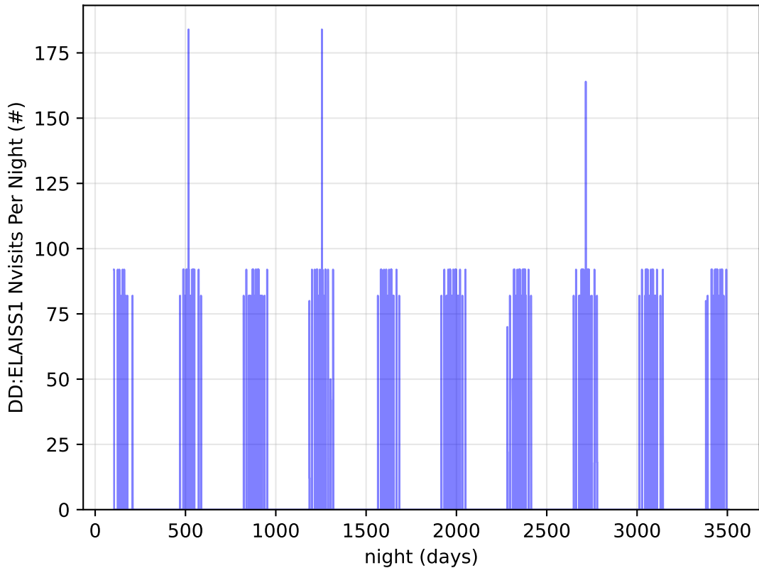
ddf_acor_sf30_lsf40_lsr20_v3.4_10yrs all bands: DD:ELAISS1 Nvisits Per Night
