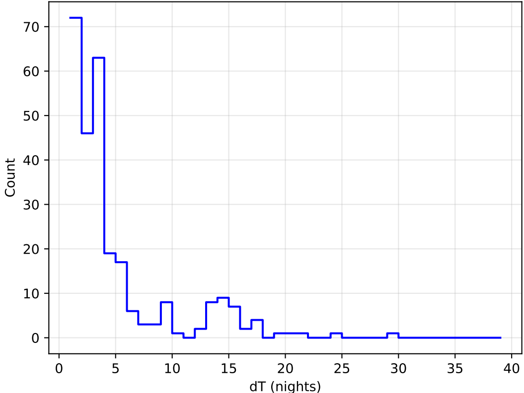
ddf_acor_sf30_lsf40_lsr20_v3.4_10yrs all bands: DD:ELAISS1 Delta Nights Histogram
