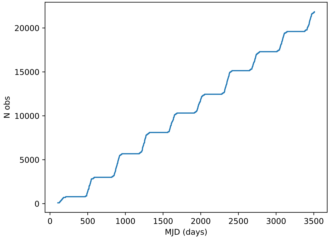
ddf_acor_sf30_lsf40_lsr20_v3.4_10yrs all bands: DD:ELAISS1 Cumulative NVisits
