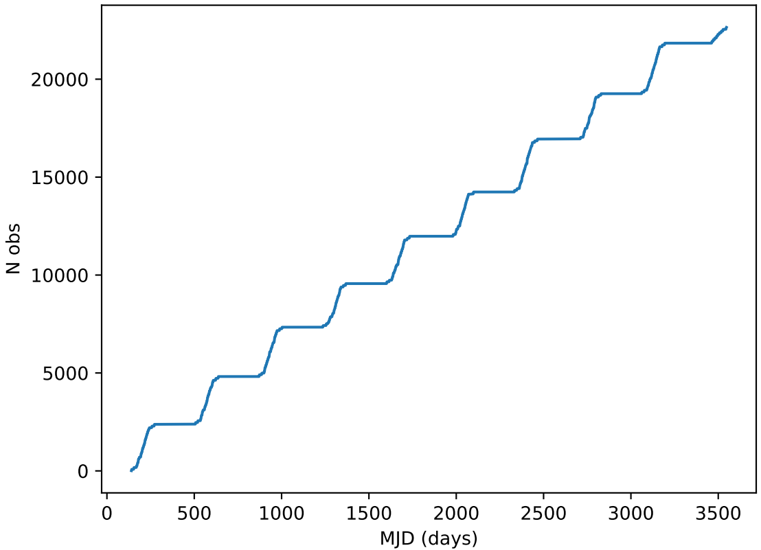
ddf_acor_sf30_lsf40_lsr20_v3.4_10yrs all bands: DD:EDFS Cumulative NVisits
