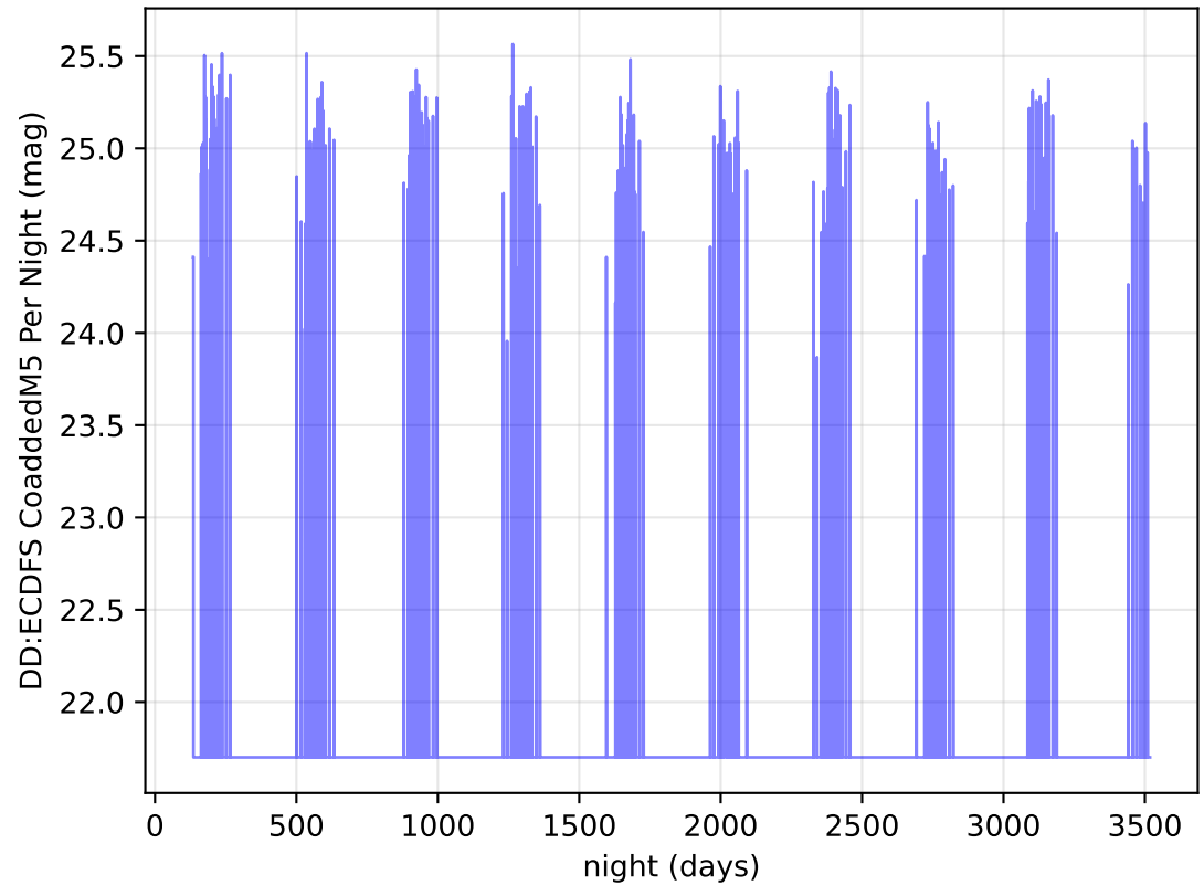
ddf_acor_sf30_lsf40_lsr20_v3.4_10yrs z band: DD:ECDFS CoaddedM5 Per Night
