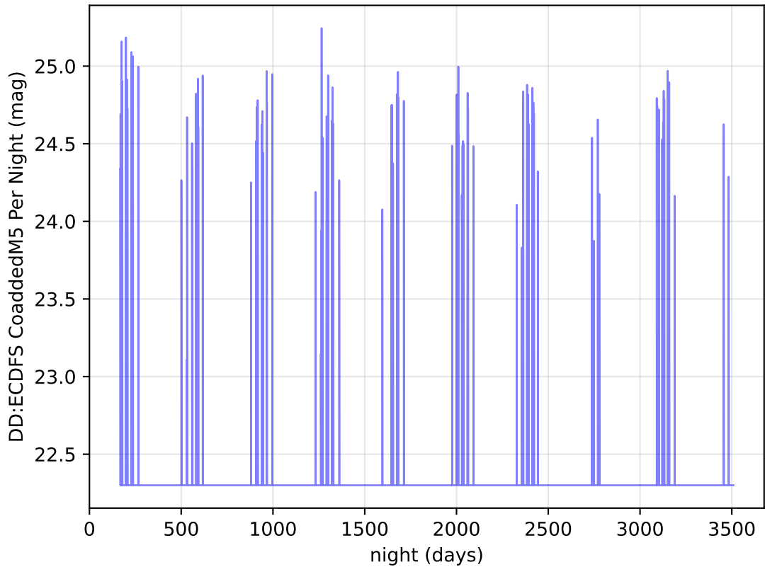
ddf_acor_sf30_lsf40_lsr20_v3.4_10yrs u band: DD:ECDFS CoaddedM5 Per Night
