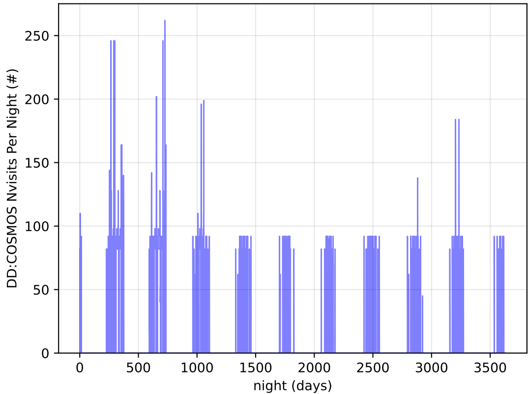
ddf_acor_sf30_lsf40_lsr20_v3.4_10yrs all bands: DD:COSMOS Nvisits Per Night
