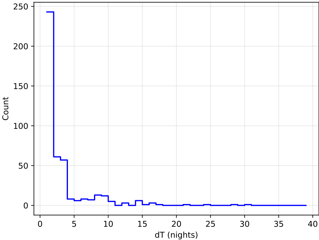
ddf_acor_sf30_Isf40_Isr20_v3.4_10yrs all bands: DD: COSMOS Delta Nights Histogram
